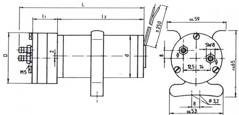
DC12/80L DC24/90L
