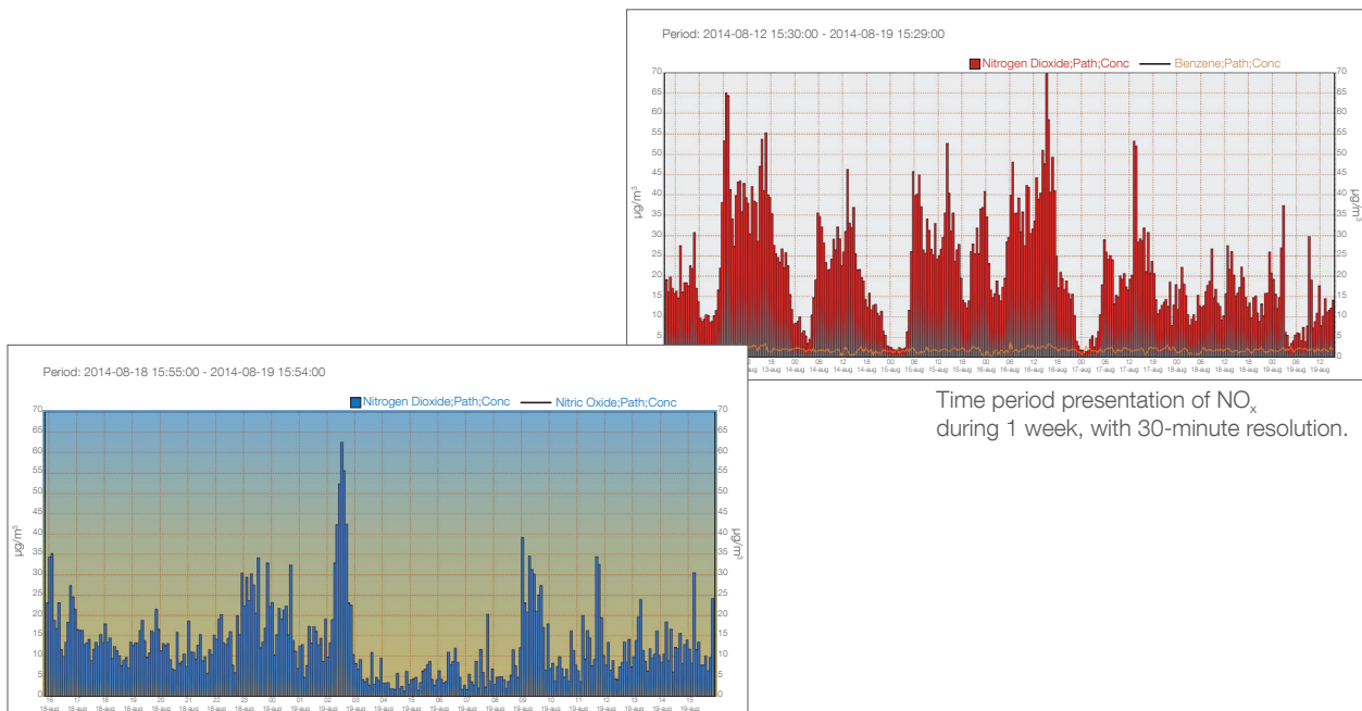
Time period presentation of \text{NO}_x during 24 hours, with 5-minute resolution.
